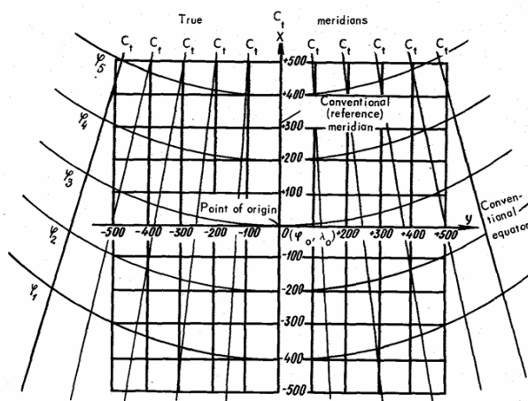
FIG. 47. EXAMPLE OF PLOTTING COORDINATE GRID FOR FLYING AREA
