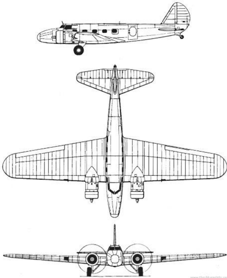
Three-view of the handsome and sleek Boeing 247. Note the thick wing which was a carry-over from past airliner designs and made necessary by the more primitive metallurgy of the 1930s. A thinner wing would have certainly added many mph to this aeroplane.
