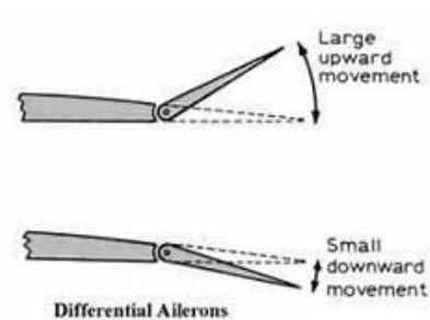
Differential Ailerons
