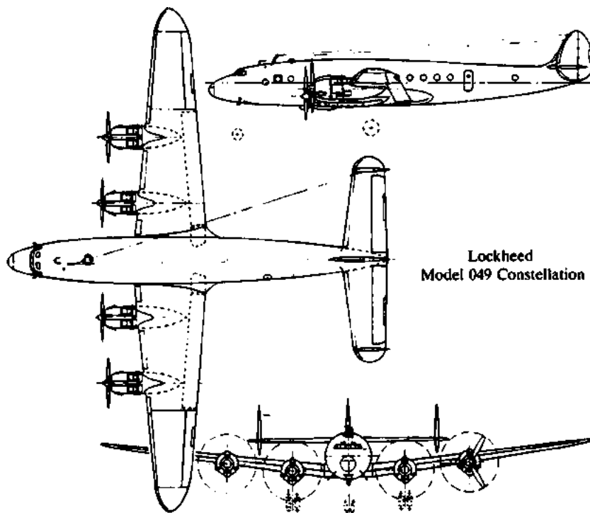
Three-view of Lockheed L-049 "Constellation". Note the circular shape of the fuselage and overall clean aerodynamic lines.
