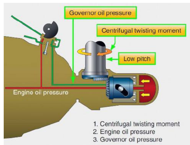
A simplified diagram of the Hamilton-Standard propeller pitch-control system.
