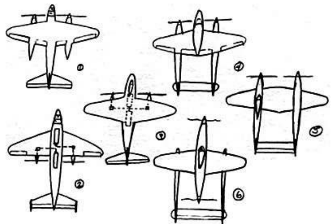
This is a copy of some of what Clarence "Kelly" Johnson's scribbled whilst trying to find a suitable form for the proposed Lockheed Model 22 which became P-38. Note that two designs (2 and 3) included engines mounted in the fuselage turning outboard propellers on the wings.
