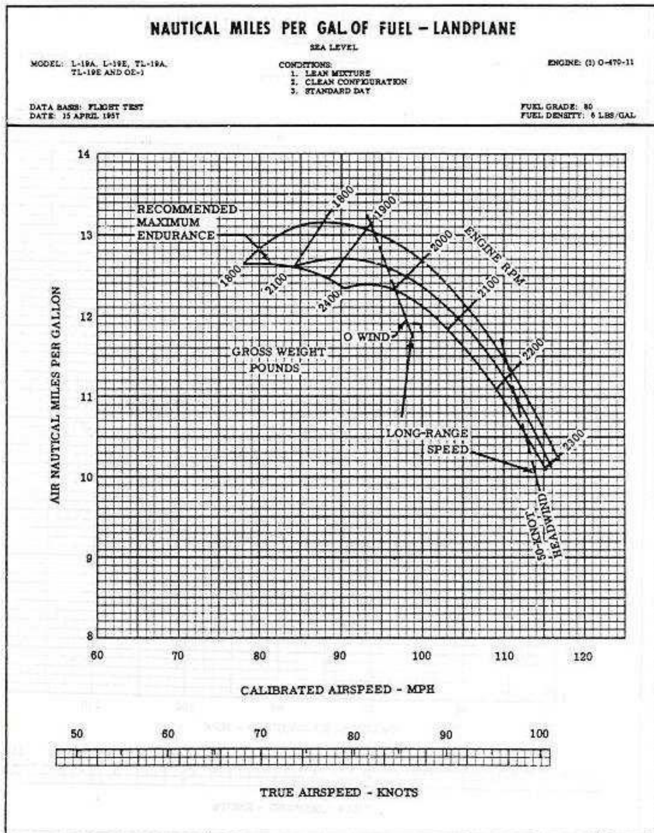
Figure 4-5 Specific Fuel Consumption / Cruise Data (Sea Level)
