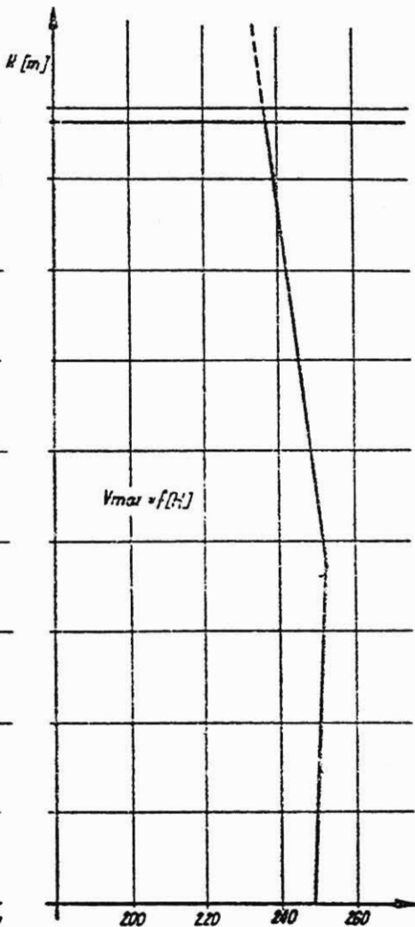
C.G. position - 24% M.A.C Diagram No. 2. Maximum Speed Versus Altitude.
