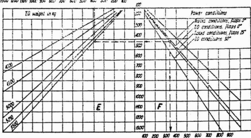
Fig. 4.7. Nomogram for Determining the Take-off Run Distance of the Airplane
