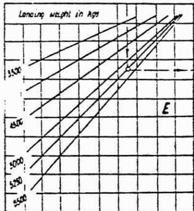
Fig. 4.8. Nomogram for Determining Airplane Landing Run Distance
