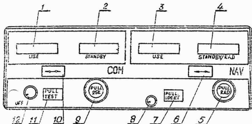
Fig. 1. KR 165 COM/NAV Transceiver
