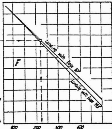
Fig. 4.8. Nomogram for Determining Airplane Landing Run Distance
