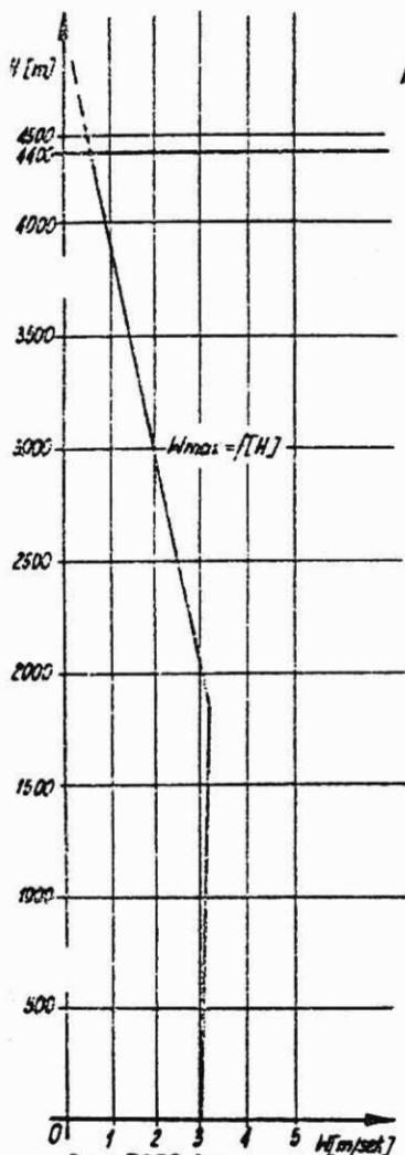
Q = 5250 kg Fig. 6-1. Diagram No. 1 Climbing Speed Versus Altitude
