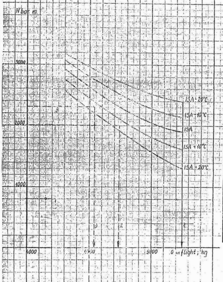
Fig. 4.12. Diagram of Maximum Acceptable Flight Weight Types 419104 and Air Temperature for the condition of ensuring climbing rate not smaller than 3.3 m/s. Rated power in engine. Airplane with agricul- tural equipment.
