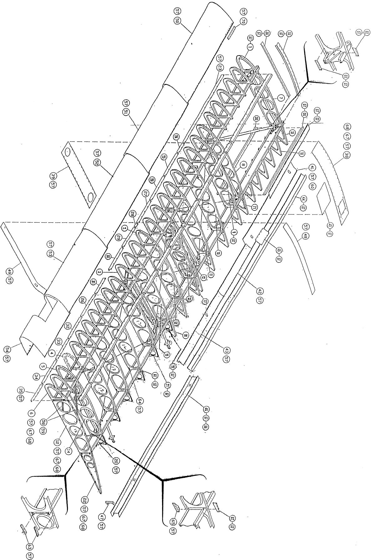
FIGURE 2 WING ASSEMBLY
