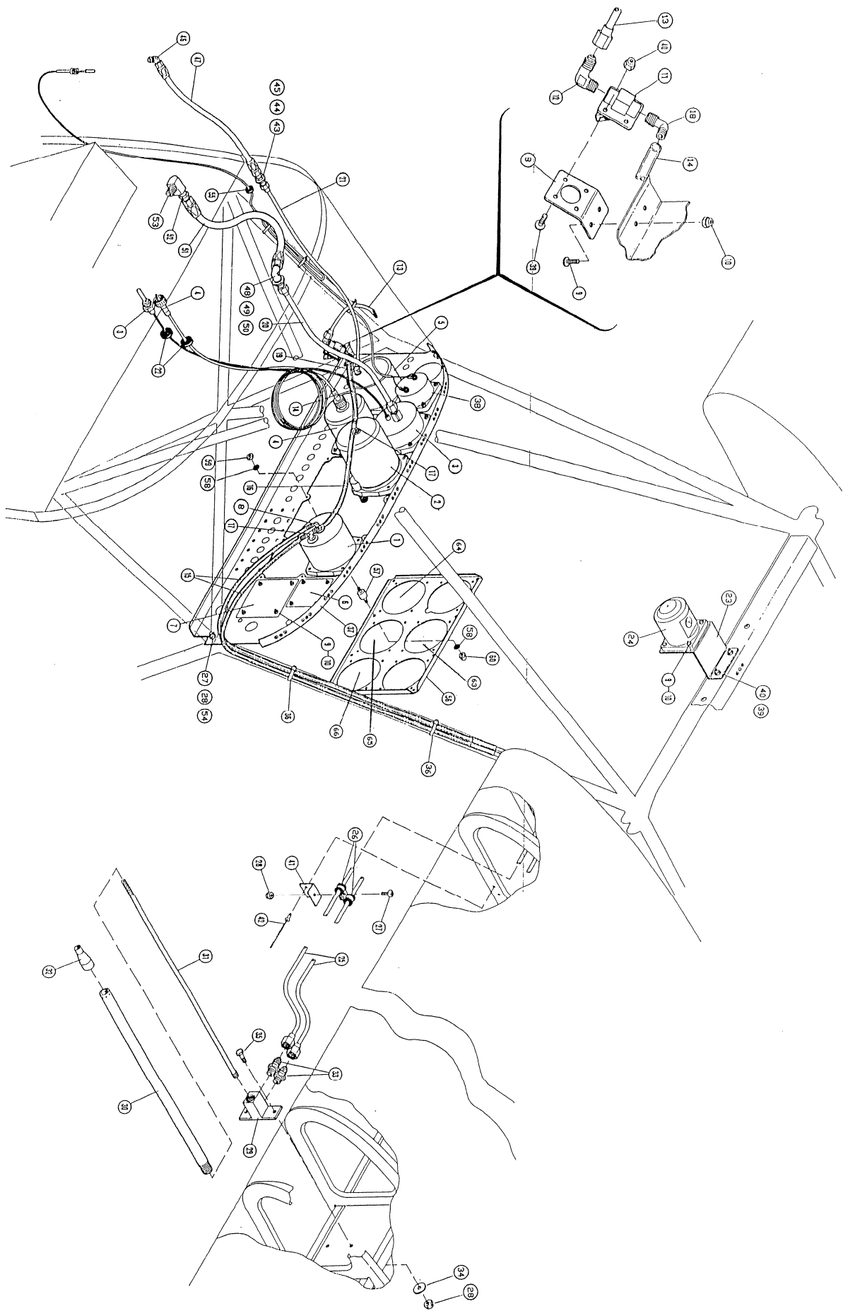
FIGURE 18: INSTRUMENTS INSTALLATION
