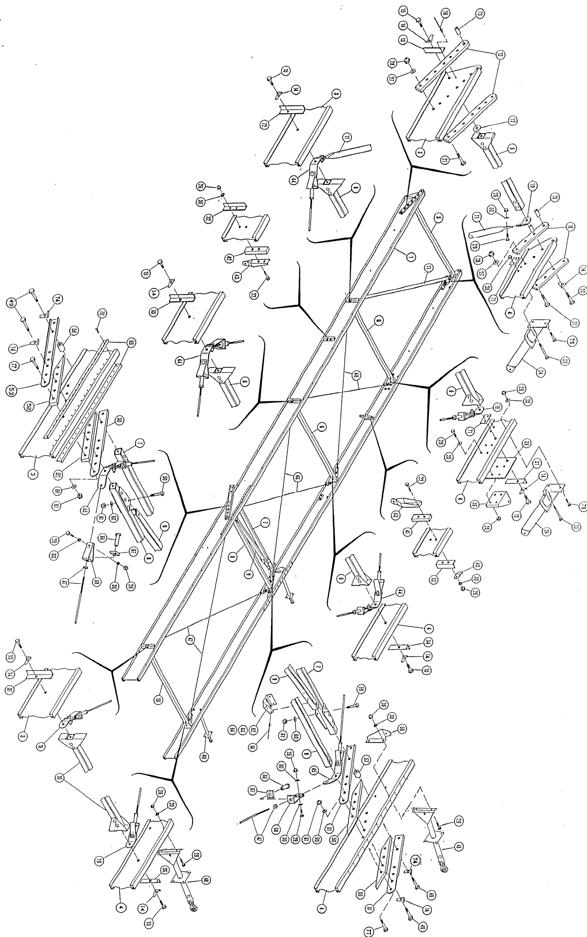
FIGURE 1: WING SPAR ASSEMBLY
