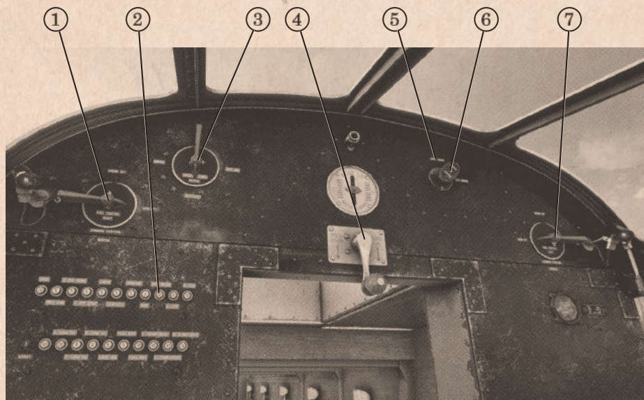
Figure 7 - Back Panel
