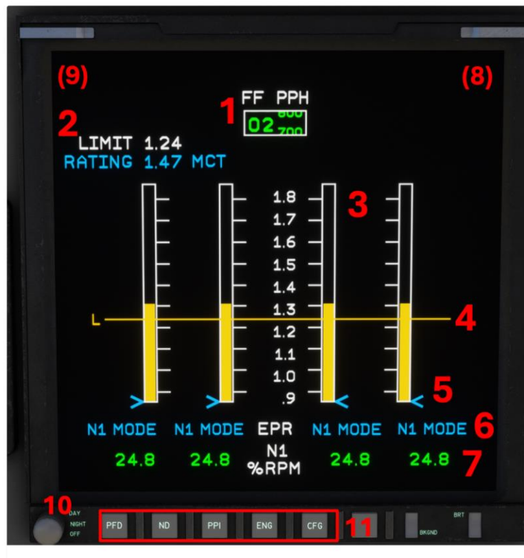
Engine Display, EPR Page
