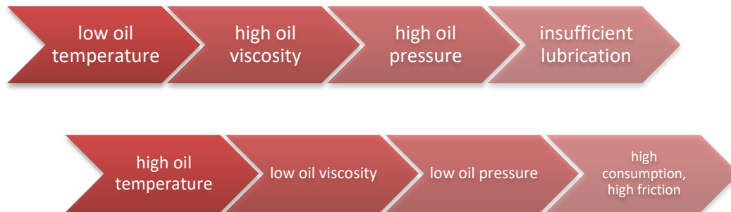
Figure 12-2: Effects of either too low or too high oil temperatures.
