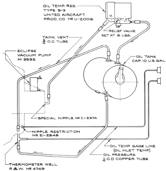
Figure 12-1: Schematic drawing of the 247D's oil system.
