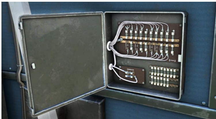
Figure 14-1: Junction box J-71, located on the right cockpit wall, contains the fuses that protect most of the ship's electrical components.
