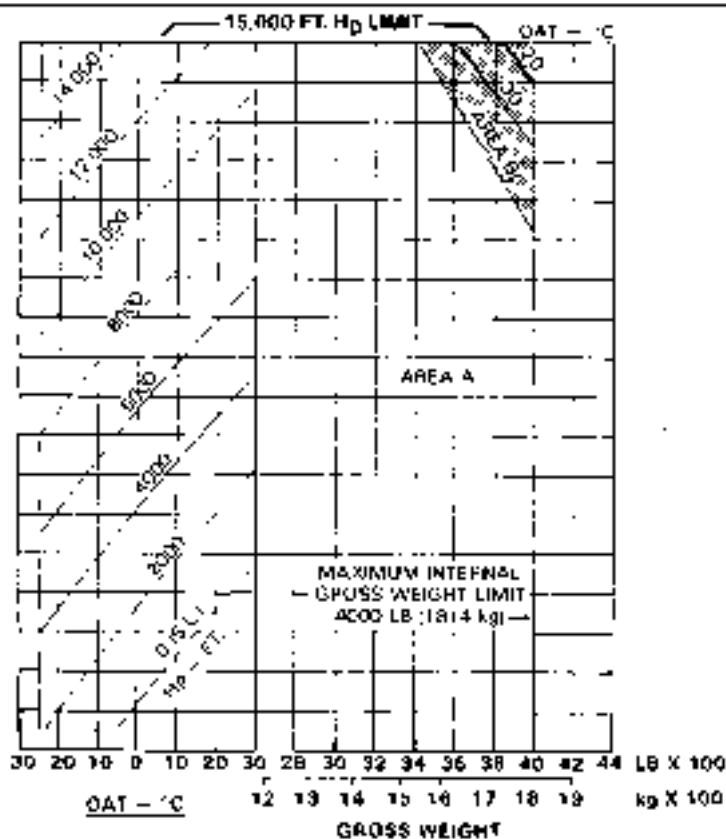
Figure 4-1. Hover ceiling (Sheet 3 of 16)
