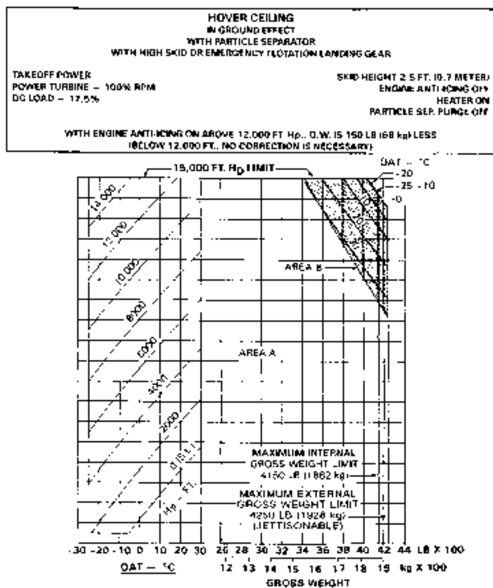
Figure 4-1. Hover ceiling (Sheet 11 of 16)
