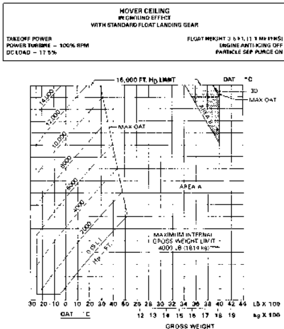
Figure 4-1 Hover ceiling in ground effect (Sheet 10 of 11)
