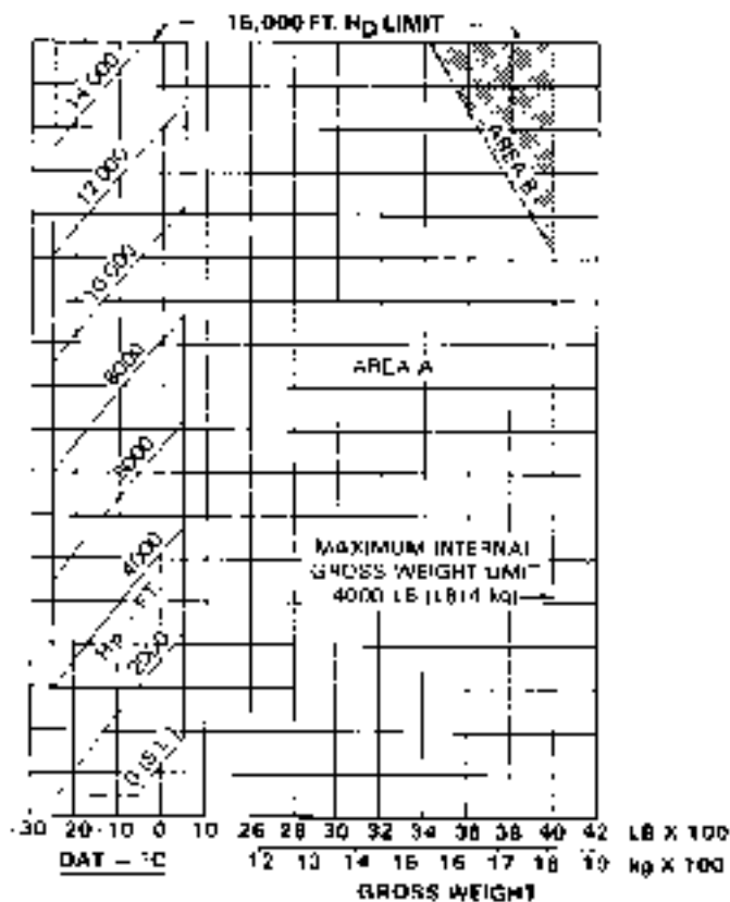
Figure 4-3. Hover ceiling — in ground effect (Sheet 5 of 6)
