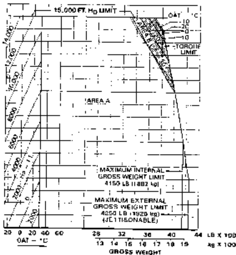
Figure 4-4. Hover ceiling — out of ground effect (Sheet 1 of 2)
