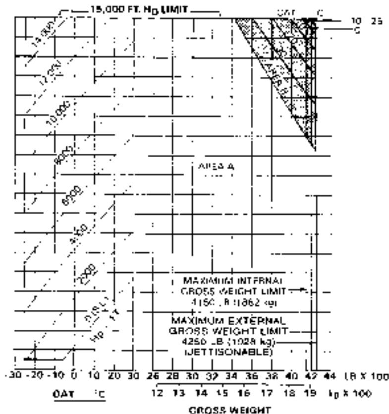
Figure 4-1. Hover ceiling (Sheet 3 of 16)
