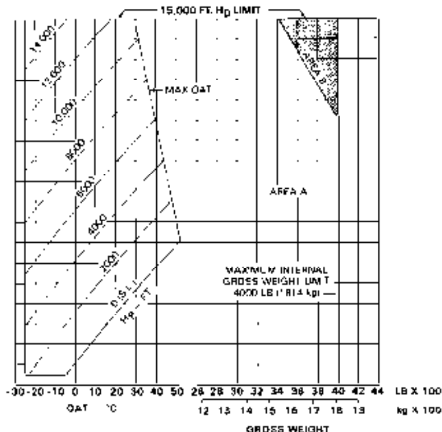
Figure 4-1. Hover ceiling in ground effect (Sheet 8 of 11)
