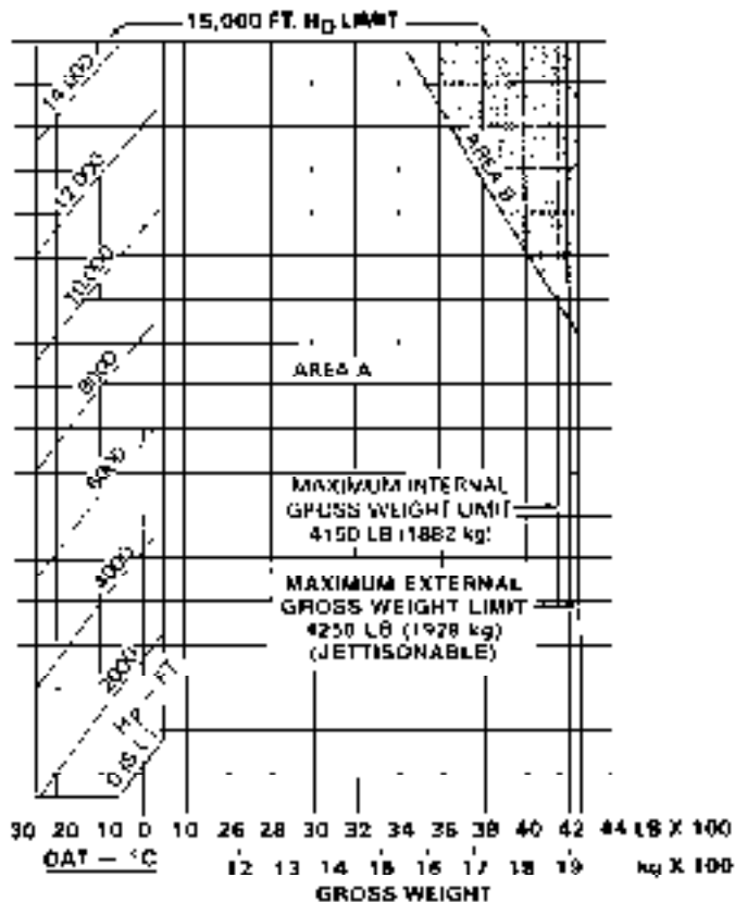
Figure 4-1. Hover ceiling in ground effect (Sheet 3 of 11)
