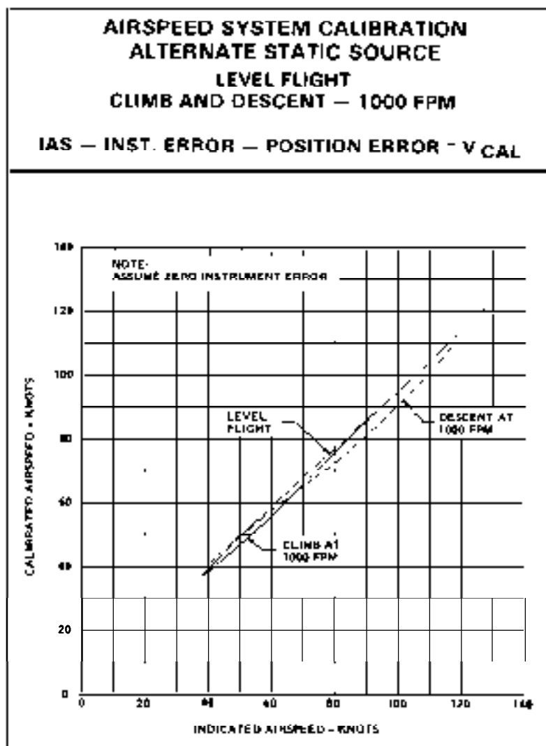
Figure 4-2. Airspeed system calibration (Sheet 2 of 2)
