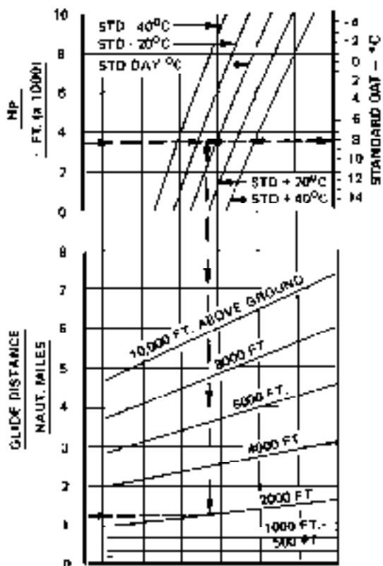
Figure 4-3. Glide distance
