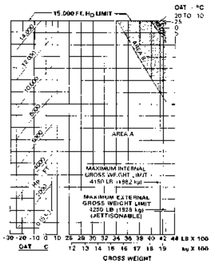
Figure 4-1. Hover ceiling in ground effect (Sheet 5 of 11)
