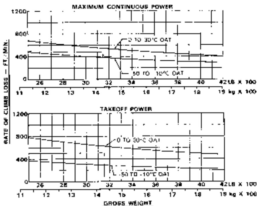
Figure 4-2. Rate of climb decrease
