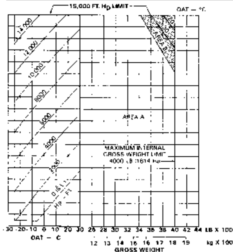
Figure 4-1. Hover ceiling (Sheet 13 of 15)
