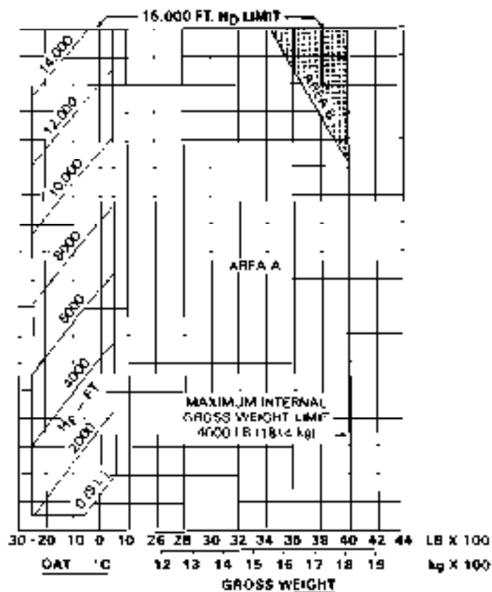
Figure 4-2. Hover ceiling in ground effect (Sheet 2 of 2)
