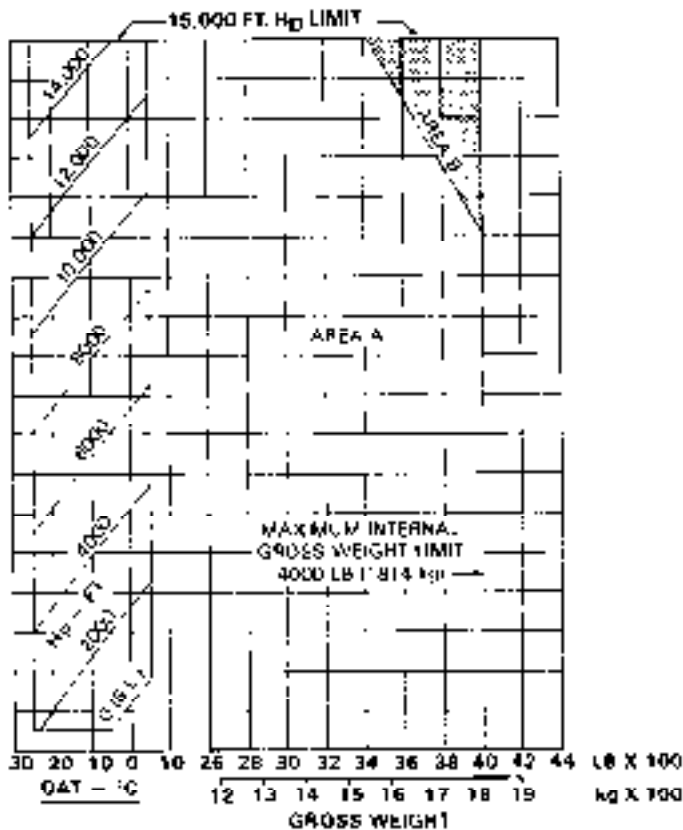
Figure 4-1. Hover ceiling in ground effect (Sheet 11 of 11)
