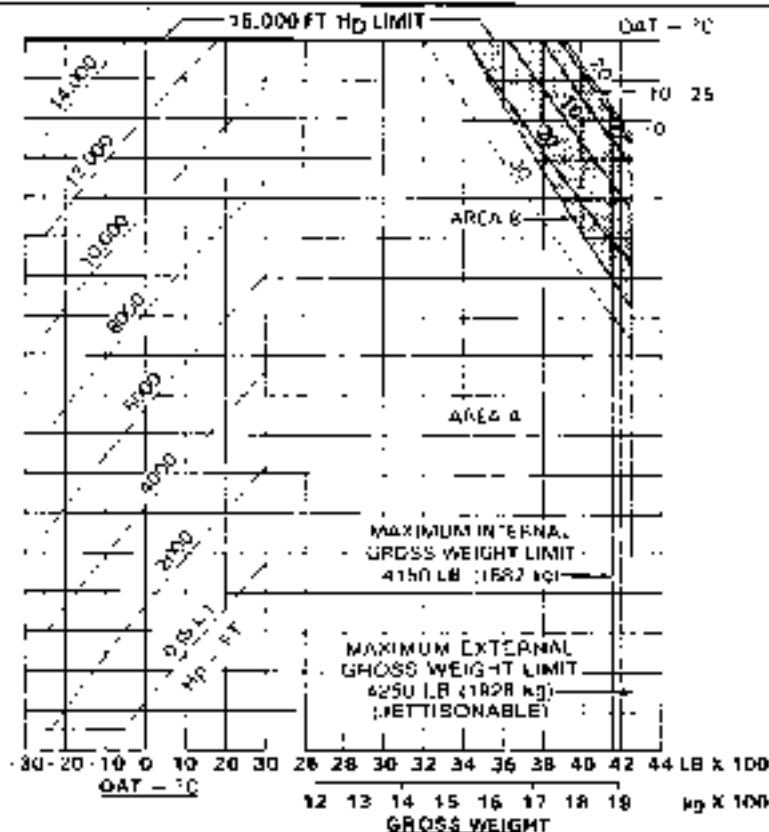
Figure 4-1. Hover ceiling (Sheet 5 of 15)
