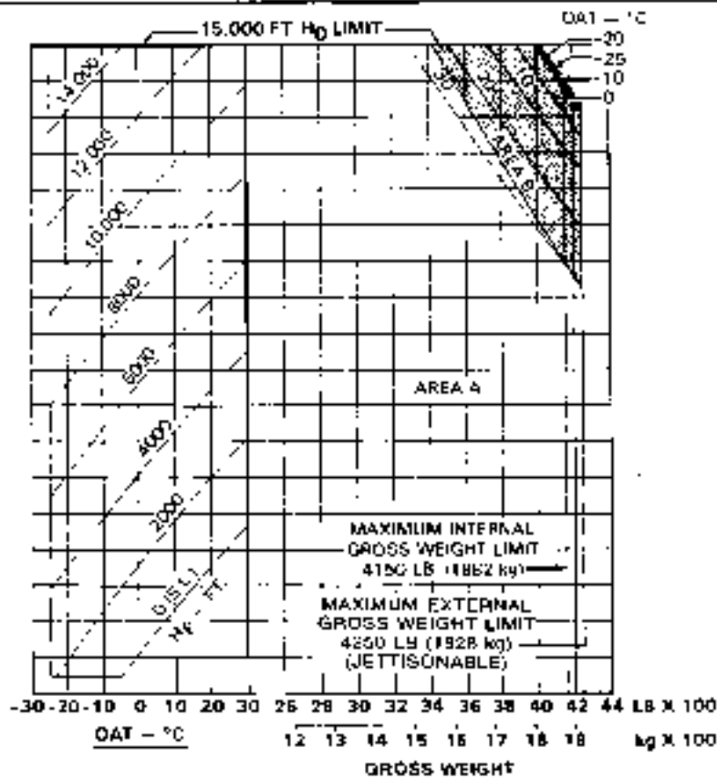
Figure 4-1. Hover ceiling (Sheet 12 of 15)
