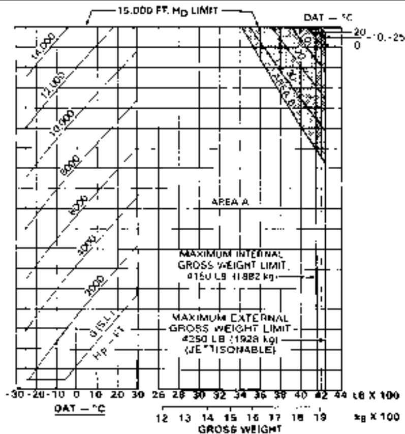
Figure 4-1. Hover ceiling (Sheet 10 of 15)
