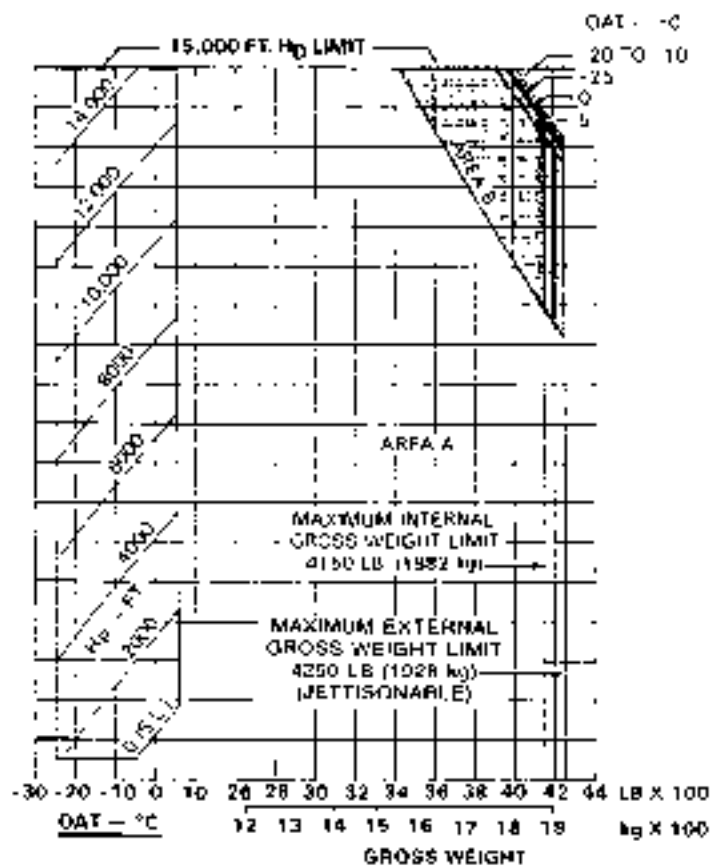
Figure 4-3. Hoyer ceiling -- in ground effect (Sheet 4 of 6)
