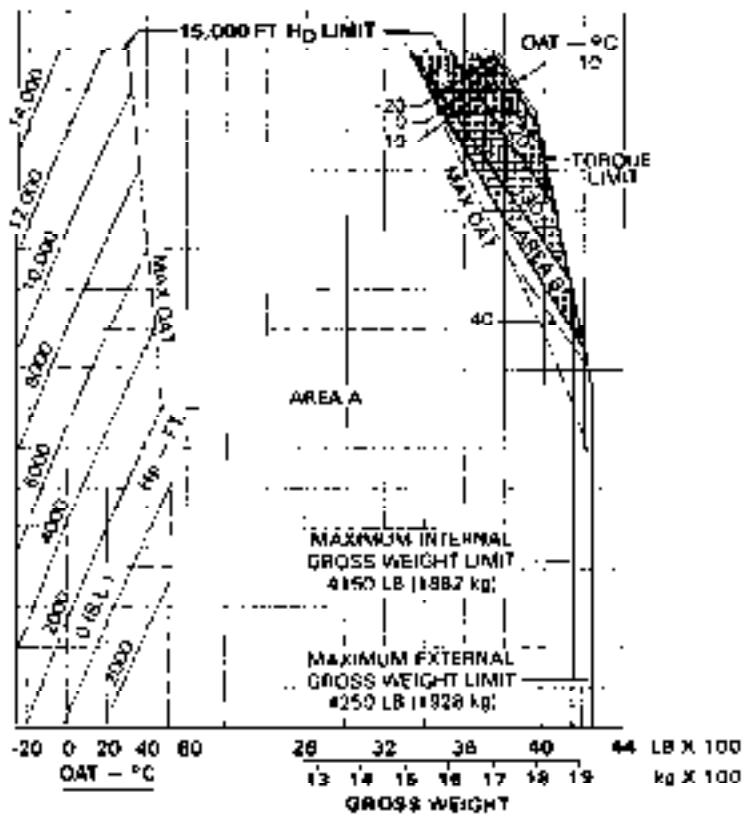
Figure 4-1. Hover ceiling out of ground effect (Sheet B of 12)
