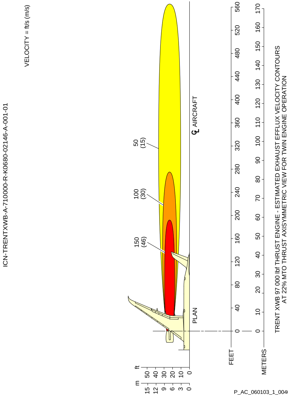
Breakaway Power (22% MTO Thrust) - TRENT XWB-97 Engine FIGURE-6-1-3-991-004-A01
