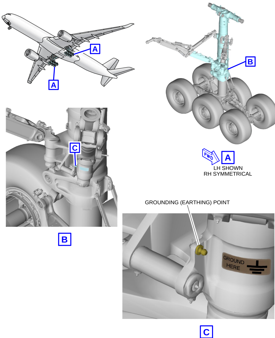
Grounding (Earthing) Point - MLG FIGURE-5-4-1-991-003-A01
